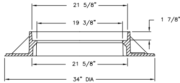
CROSS SECTION
